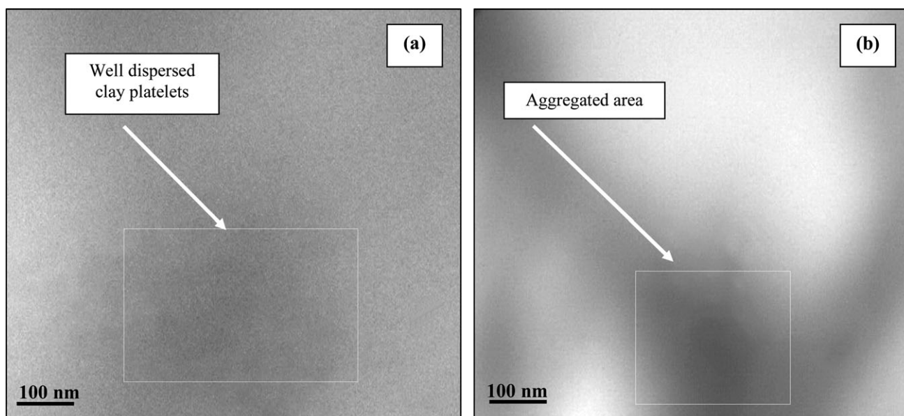
Figure 4. TEM micrographs of WPCs types of B2 (a) and B3 (b).
